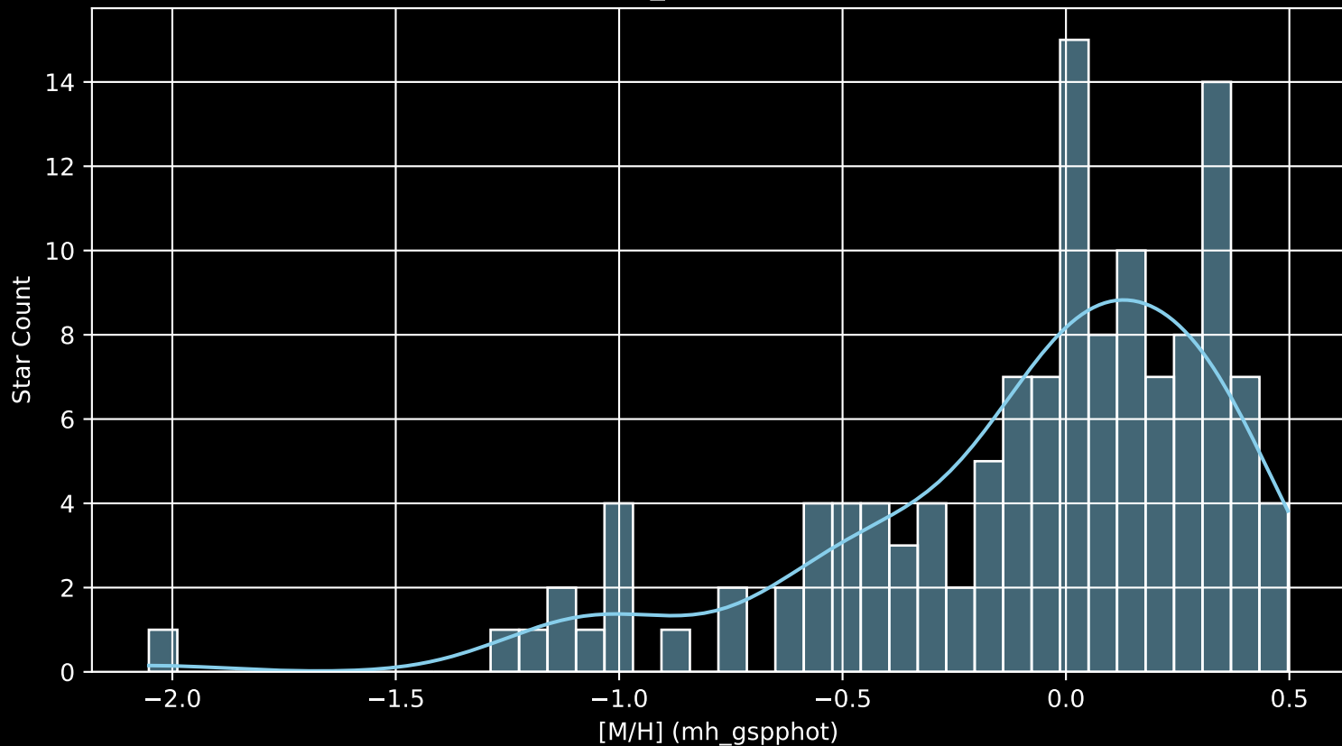
APOGEE DR17 Field: [060+00_btx [M/H] (mh_gspphot) (n= 128)
