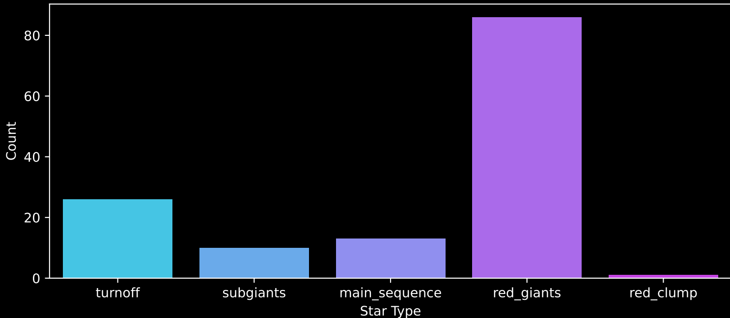
APOGEE DR17 Field: [060+00_btx] Count plot of Star Type
