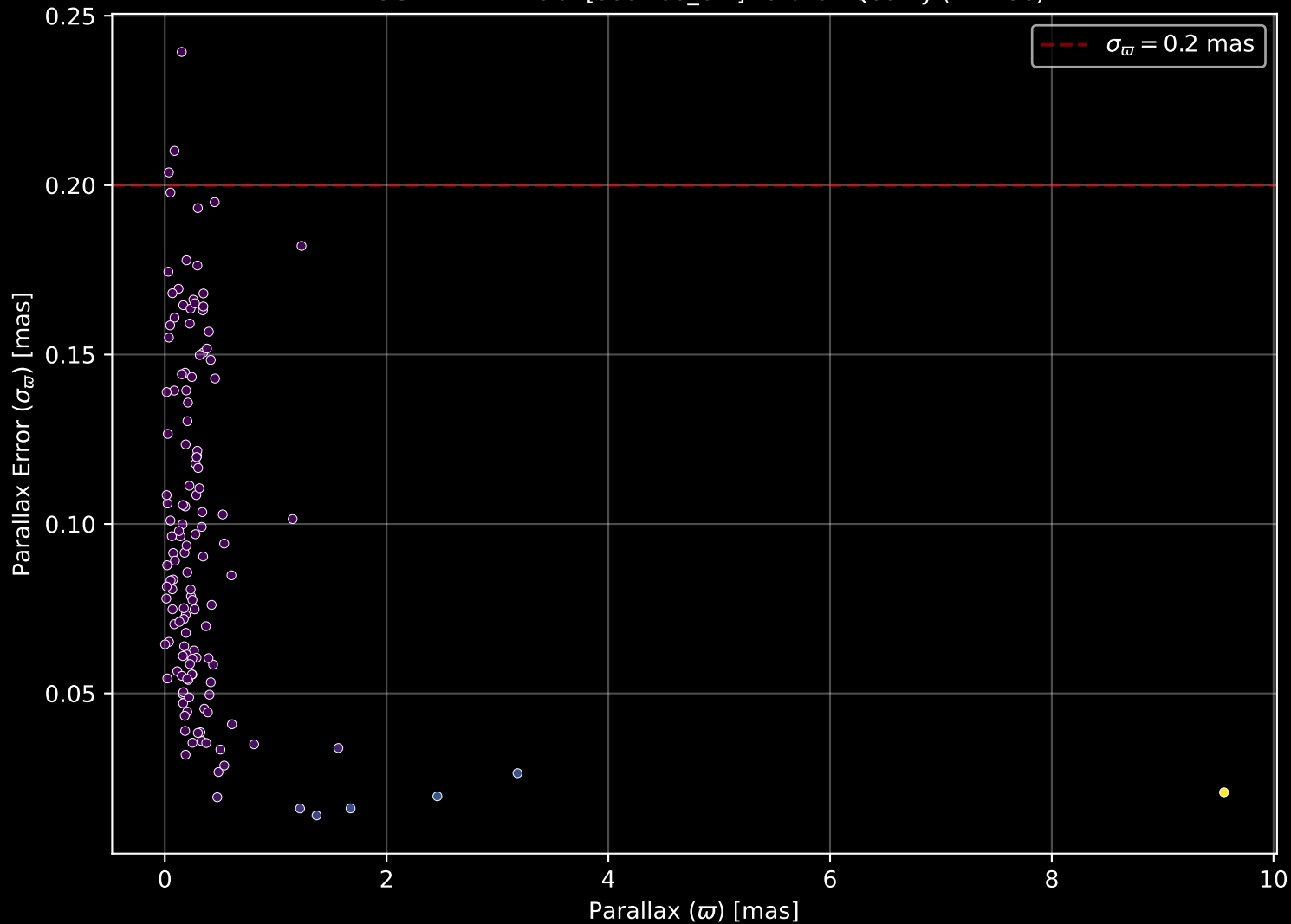
APOGEE DR17 Field: [060+00_btx] Parallax Quality (n= 136)
