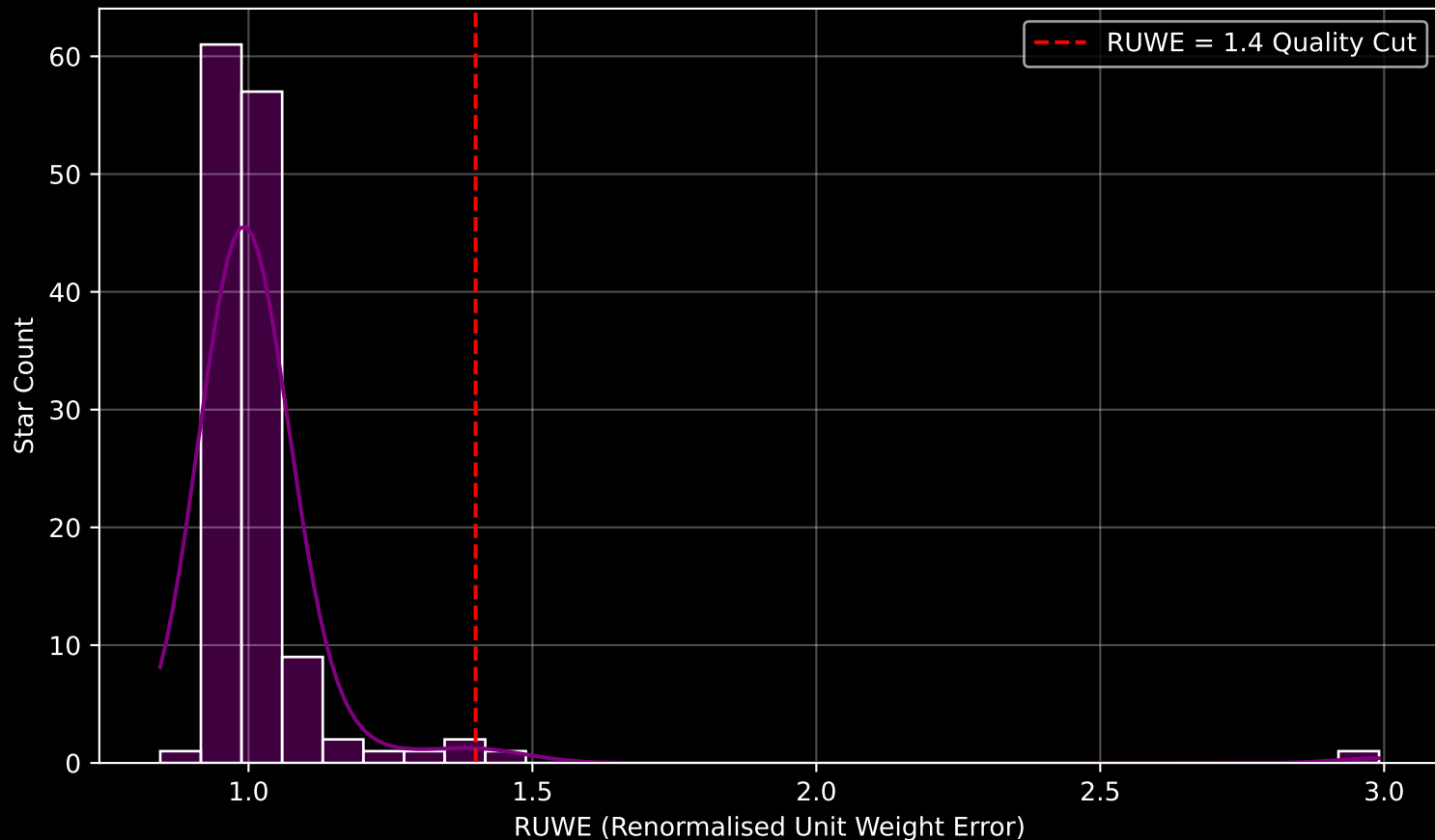
GAPOGEE DR17 Field [060+00_btx] RUWE Distribution (n= 136)
