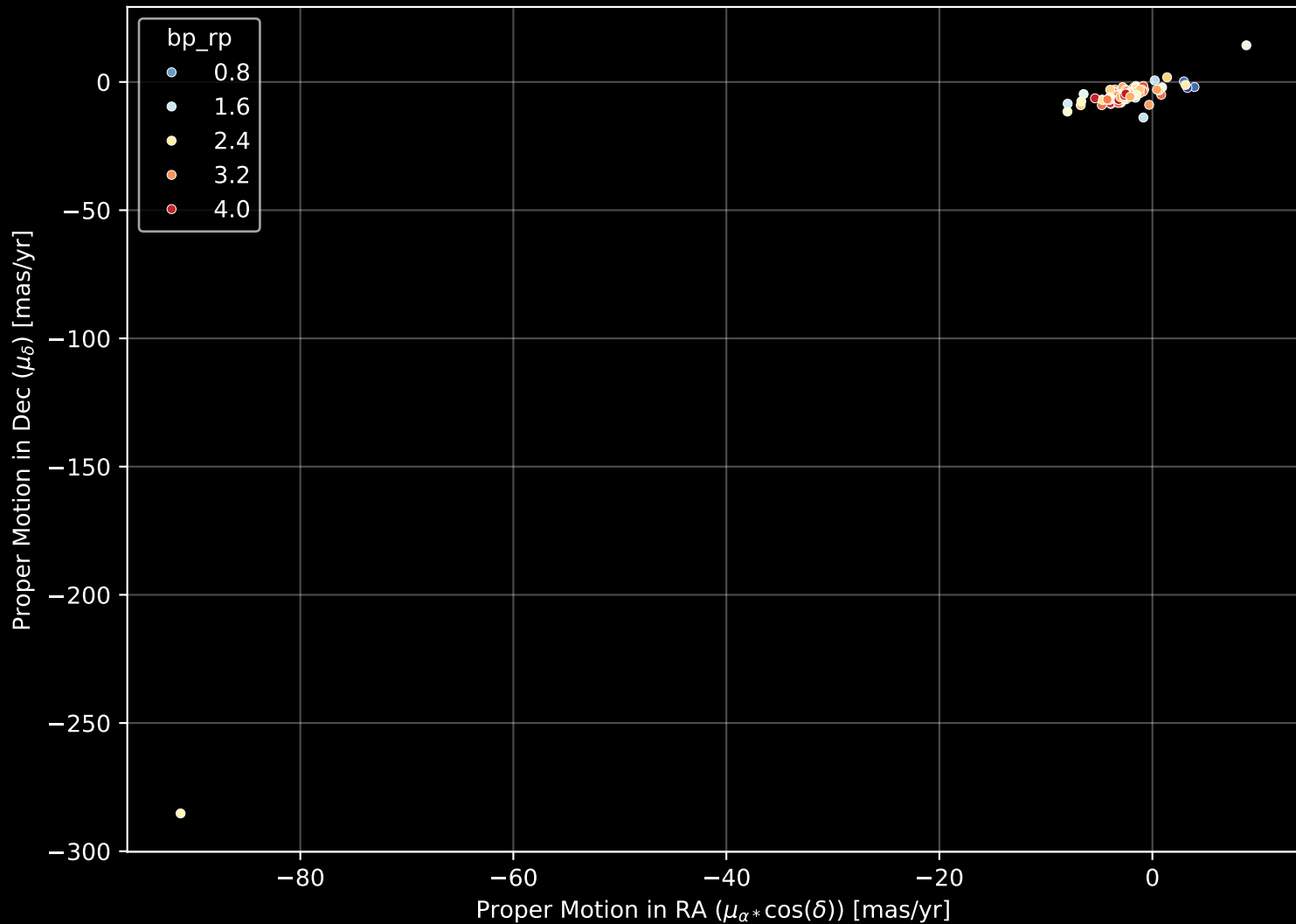
APOGEE DR17 Field: [060+00_btx] Proper Motion Diagram (n= 136)
